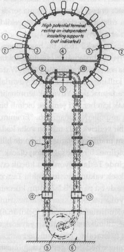
FIG. 4 SCHEMATIC ILLUSTRATION OF NEW HIGH POTENTIAL GENERATOR
