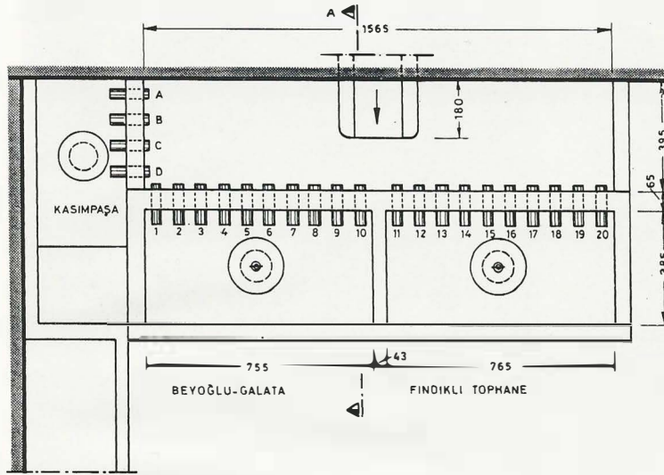
Taksim Distribution Chamber and discharge measuring system
