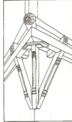
111 Ahşap payandalar
