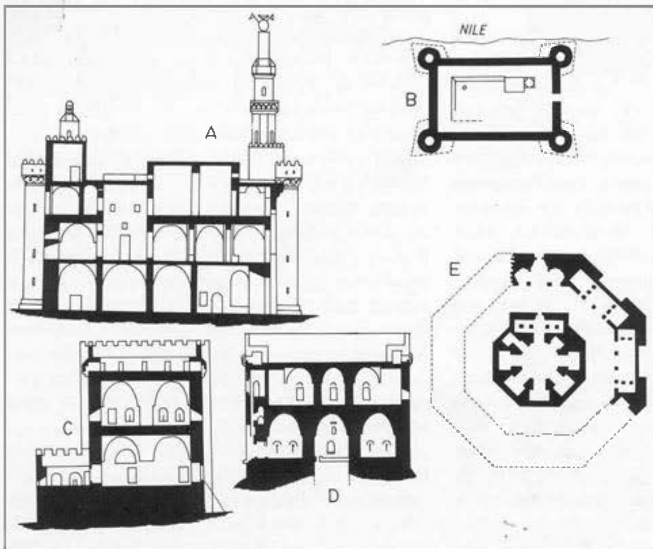
(A) Section through the central keep and mosque of Qayt-bay's fortress overlooking Alexandria harbour, 1479. (B) Plan of Qayt-bay's small fort overlooking the Nile north of Rashid, 1479 (after De Cusson). (C) Restored section through the 'Rivermouth Tower', Tripoli, Lebanon, c.1475, with additional bastion on left dating from the 17th-18th cents. (after Sauvaget). (D) Section through the 'Lions Tower', Tripoli, Lebanon, c.1475 (after Sauvaget). (E) Plan of the Qal'at al Tina, Simi, probably built for Sultan al Ghuri in the early 16th cent. (after Tamari).
