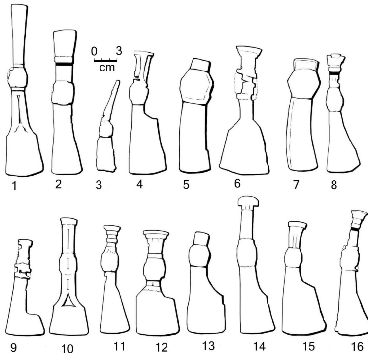
Khazar axeheads: (1, 5, 8, 11, 14 & 16) from Sukhaya Gomolsha; (2 & 13) from Netaylovka; (3) from Borisovo; (4) from Topoli; (6, 9 & 12) from Krasnaya Gorka; (7) from Zheltoe; (10) from Kochetok; (15) from Lysiy Gorb. (Drawings by A. Karbivnychi after V. Kriganov)
