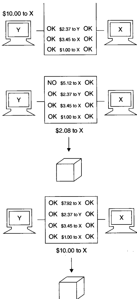
FIGURE 11.2 Two computers in the network open up a transaction, like a small box. Little by little, transactions add up within it until it uses up the entire value of the transaction, and then it is closed, and sent to the network. Each mini transaction appears as a small agreement, requiring both computers' consent.
