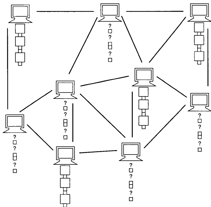
FIGURE 11.1 Two different halves of the same network. One produces a blockchain that includes both small blocks and big blocks. The other side sees the same blockchain, except that it cannot see the big blocks, only the small blocks. Therefore, it creates a second blockchain, without any big blocks at all.
