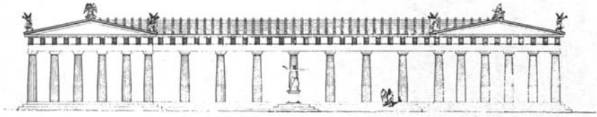
Fig. 29. Restoration of the façade of the Stoa of Zeus, Athens. (After H. A. Thompson, Hesperia 6 (1937) 54, fig. 34; cf. Coulton 1976 (1950) fig. 8.)
