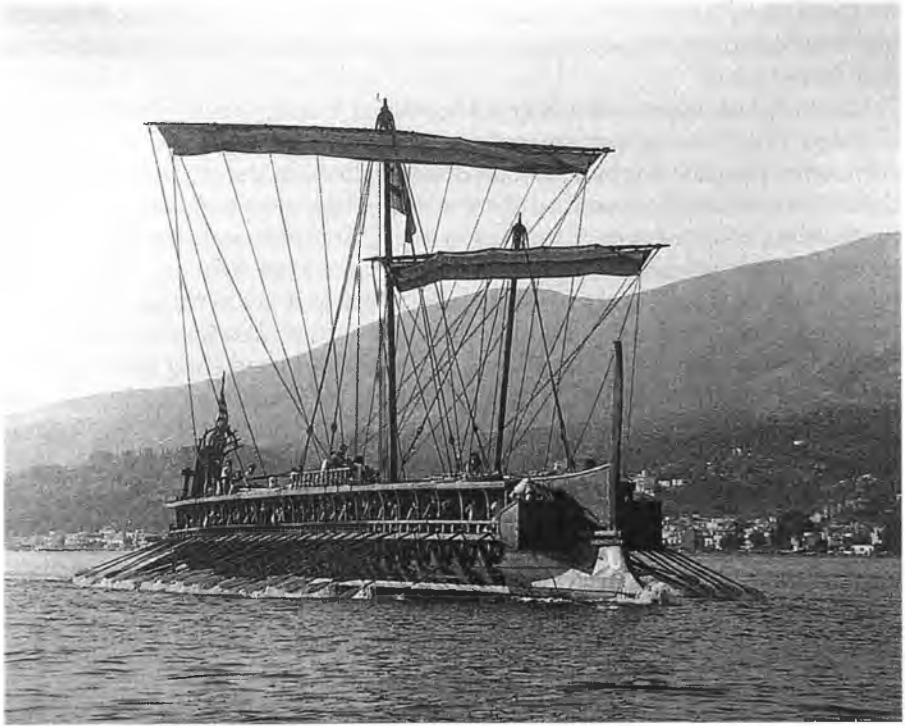
The trireme Olympias is a modern reconstruction designed by naval architect John Coates and built by the Greek navy in 1987. Triremes carried sails and used them to travel long distances, but in battle they were rowed by a large crew, as here. (Photo by Alexandra Guest, courtesy of the Trireme Trust)
