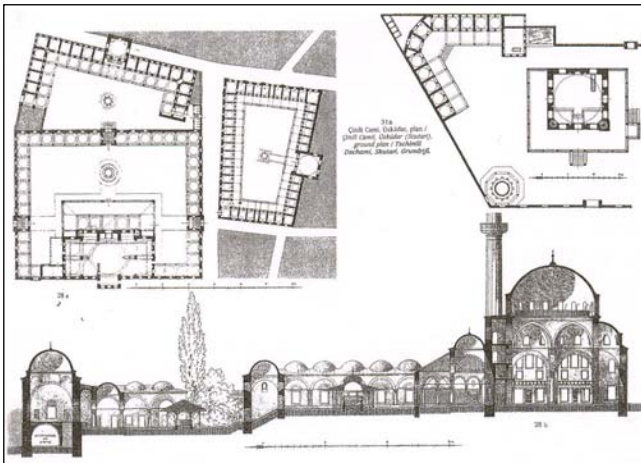
Figure 6: Atik Valide complex, plan of mosque, medrese and hankah, section of mosque and medrese (from Gurlitt).
