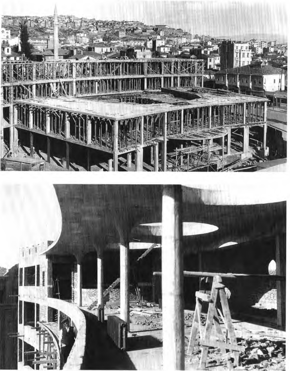
Fig. 3.18. Construction photographs of the Sümerbank building by Martin Elsaesser. Top: May 1937, midway through construction, showing the enormous scale of the building with respect to the urban fabric of old Ankara around the citadel. Bottom: September 1937 view of the top floor under construction, showing the reinforced concrete mushroom columns and circular skylights.
