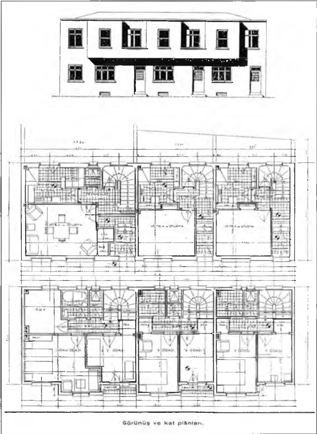
Fig. 5.19. Project for “economical prototype family houses for Ankara” by Seyfi Arkan (1933). Fig. 5.20. Project for row houses by Tahir Turan (1934) showing the influence of “Ankara cubic” on the façade articulation (see fig. 4.8).
