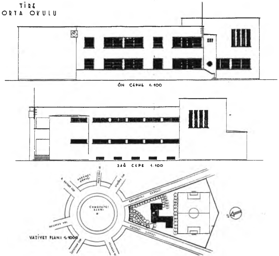
Fig. 2.21. A representative example of modernist school design in the 1930s: project for a middle school in Tire by Abidin Mertaş, as published in Arkitekt , 1937. Different functions are grouped in different blocks in an L-shaped layout defining an outdoor assembly area. Flat roofs and undecorated cubic volumes reflect a distinctly modernist aesthetic. Different window sizes and forms of windows reflect what is behind them: large windows for the classrooms, narrow horizontal bands for corridors, circular windows and/or vertical slits for stair shafts and double-height spaces such as the gym.
