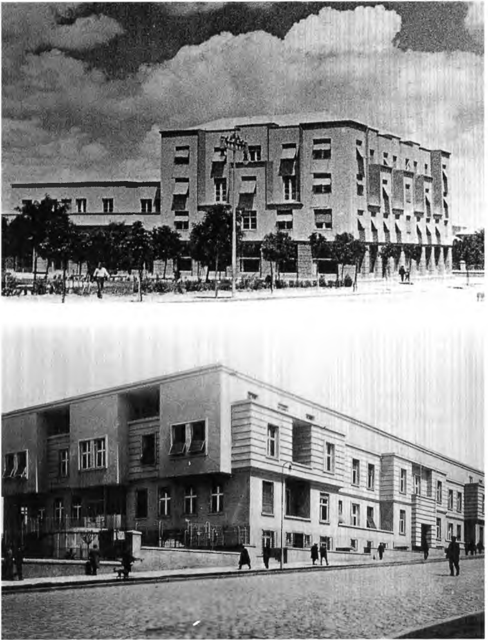
Fig. 4.8. The so-called Ankara cubic or Viennese cubic style of Ankara's major public buildings. Top: Officers' Club (1929–1933), by Clemenz Holzmeister. Bottom: Court of Financial Appeals (1928–1930), by Ernst Egli. The inverted T-shaped projections of Holzmeister and the cubic window projections of Egli were distinct leitmotifs of this style.
