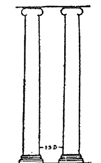
PYCNOSTYLE COLUMN ACCORDING TO VITRUVIUS
