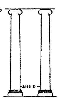
COLUMN FROM THE TEMPLE AT TEOS (HEIGHT AS GIVEN BY R. P. VALLAT)
