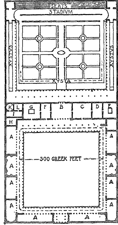
I. THE PALAESTRA AT OLYMPIA II. THE GREEK PALAESTRA ACCORD- ING TO VITRUVIUS
