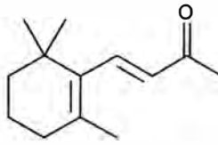
\beta -ionone
