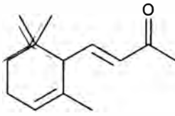
\alpha -ionone
