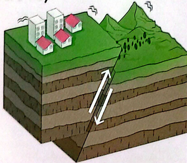
Ters Fay
