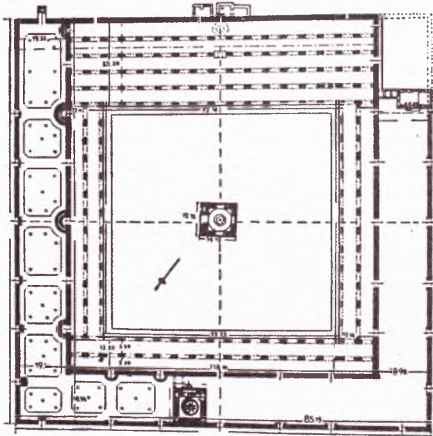
38. Kahire. İbn Tulun Camii, 876-879, plan (Dietrich Brandenburg, İslamische Baukunst in Aegypten ’den alınma).
