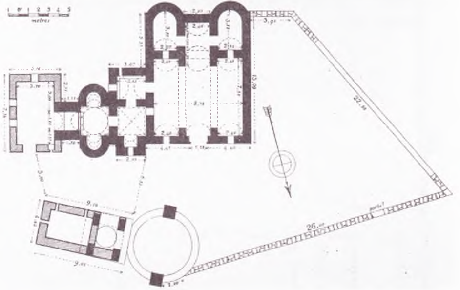
59. Kuseyr Amra. Hamam, plan
