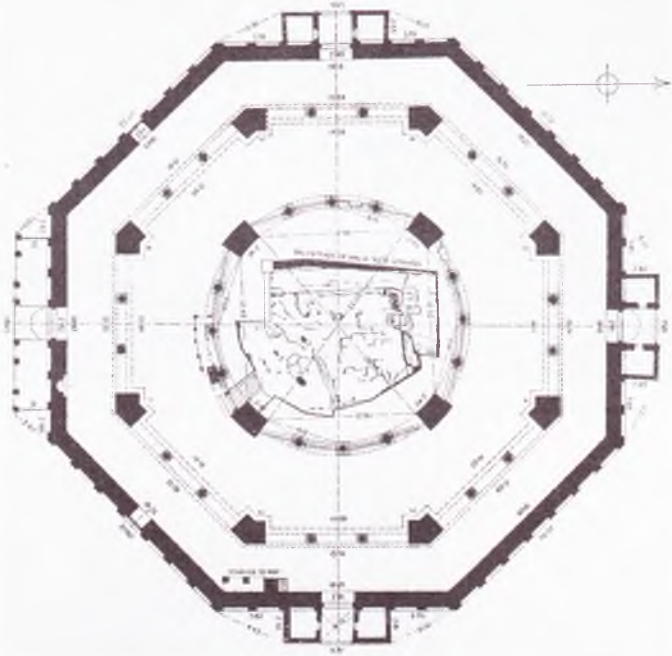
6. Kubbetü's-Sahra, plan (K. Archibald C. Creswell, Early Muslim Architecture , cilt II'den alınma).
