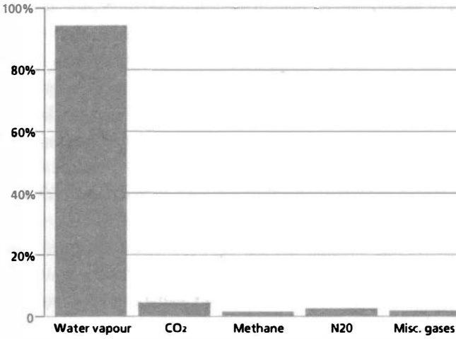
Contribution to the Greenhouse Effect (including water vapour)
