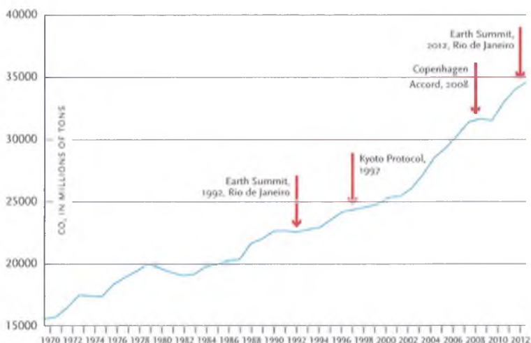
Global CO 2 Emissions, 1970–2013
