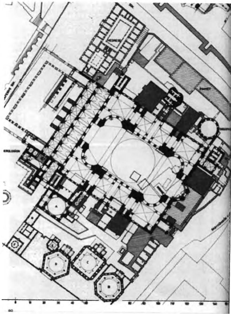
ILLUSTRATION FIVE: THE GROUNDPLAN OF HAGIA SOPHIA
