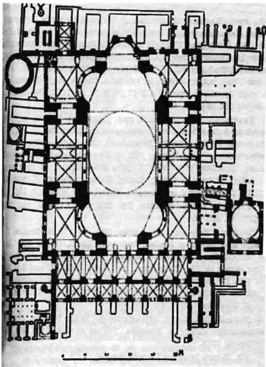
ILLUSTRATION SIX: THE GROUNDPLAN OF HAGIA SOPHIA
