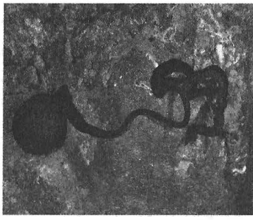
Bonellia
