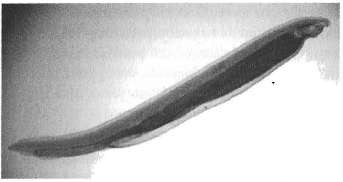
Amphioxus ( www//htt.pwholemoust-fabian-2 ).
