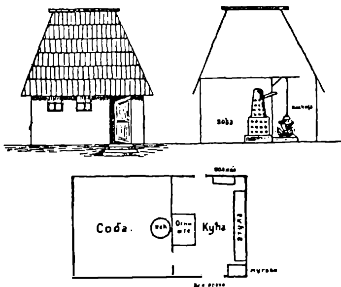
Fig. 4 Plan and section of a Serb house of Bosnia after R. Meringer
