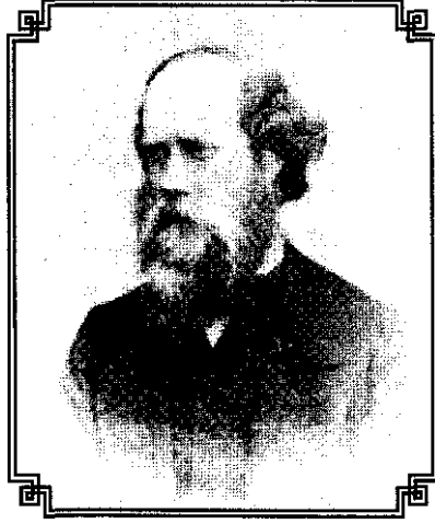
Henry Smith (1826-1883)
