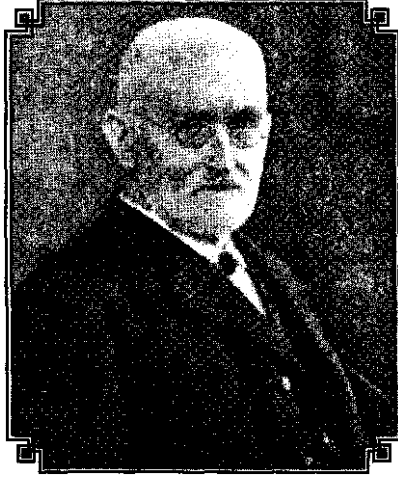
Richard Dedekind (1831-1916)
