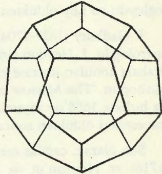
Dodekahedron
