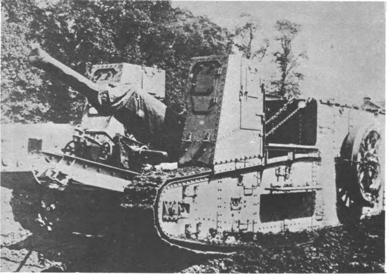
İngiliz gun-carrier tank
