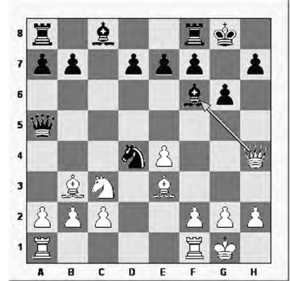
Nezhmetdinov-Chernikov, 1962
