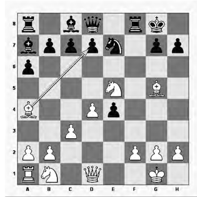
Neikirich-Radulov, 1964
