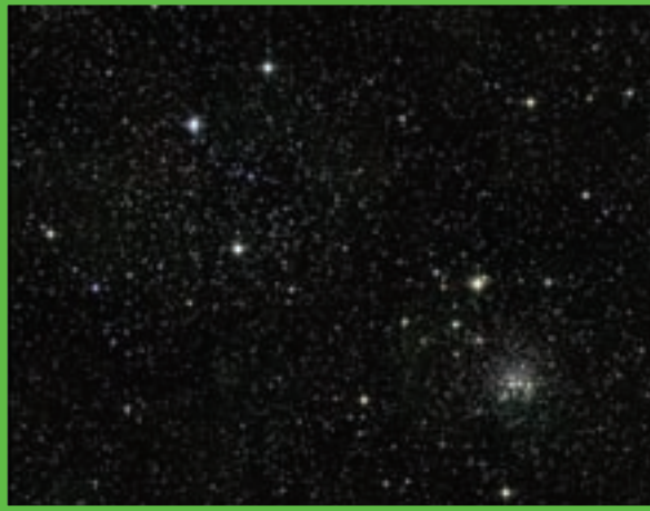
2MASS/UNMass/IPAC-Caltech/NASA/NSF
