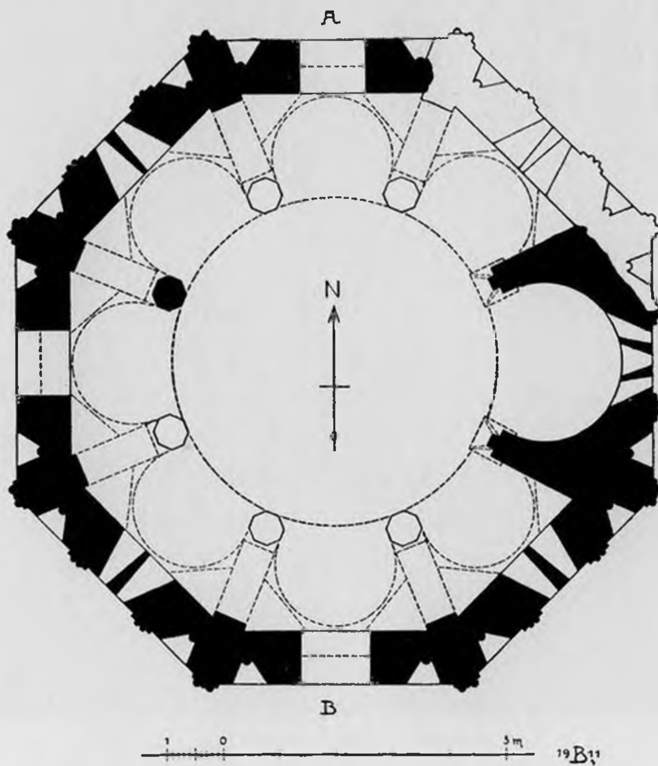
III. 5. Diagram of Octagonal Church, Varzahan
