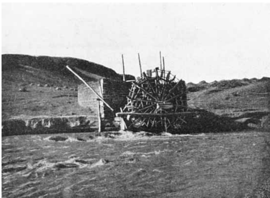
2. Waterwheel near Çokgöz bridge, on the Kızılırmak (ancient Halys, central Anatolia). This photograph from the late nineteenth century shows the principal source of energy used in milling, but also for the manufacture of gunpowder. That many Anatolian rivers carried sufficient water for milling only during certain months of the year proved a serious constraint on manufacturing.
