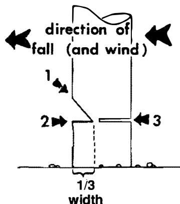
Chainsaw felling; note sequence of cuts.
